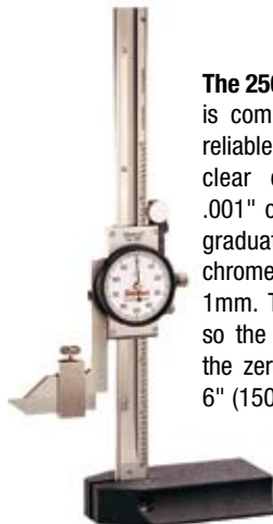
250-6 Dial Height Gage
