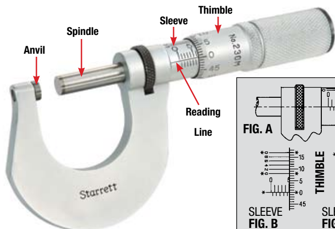
Starrett No. V230MXFL Outside Micrometer.
