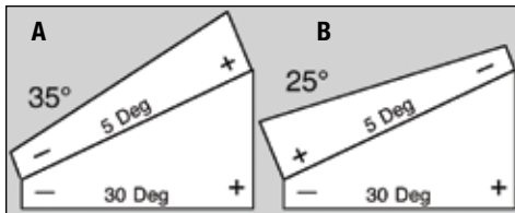
Sketches illustrate how angles of 35° and 25° can be obtained using only two angle gage blocks.
