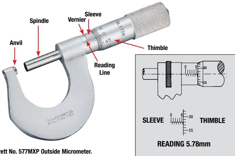
Starrett No. 577MXP Outside Micrometer.
