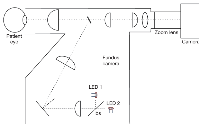
Figure 1 The layout of the FOS Device. All light sources were replaced with controllable LED systems. The imager consisted of a fundus camera combined with a zoom lens. FOS, Flow Oximetry System; LED, light emitting diode.
